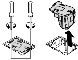
Securing screws
