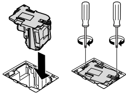
Securing screws
